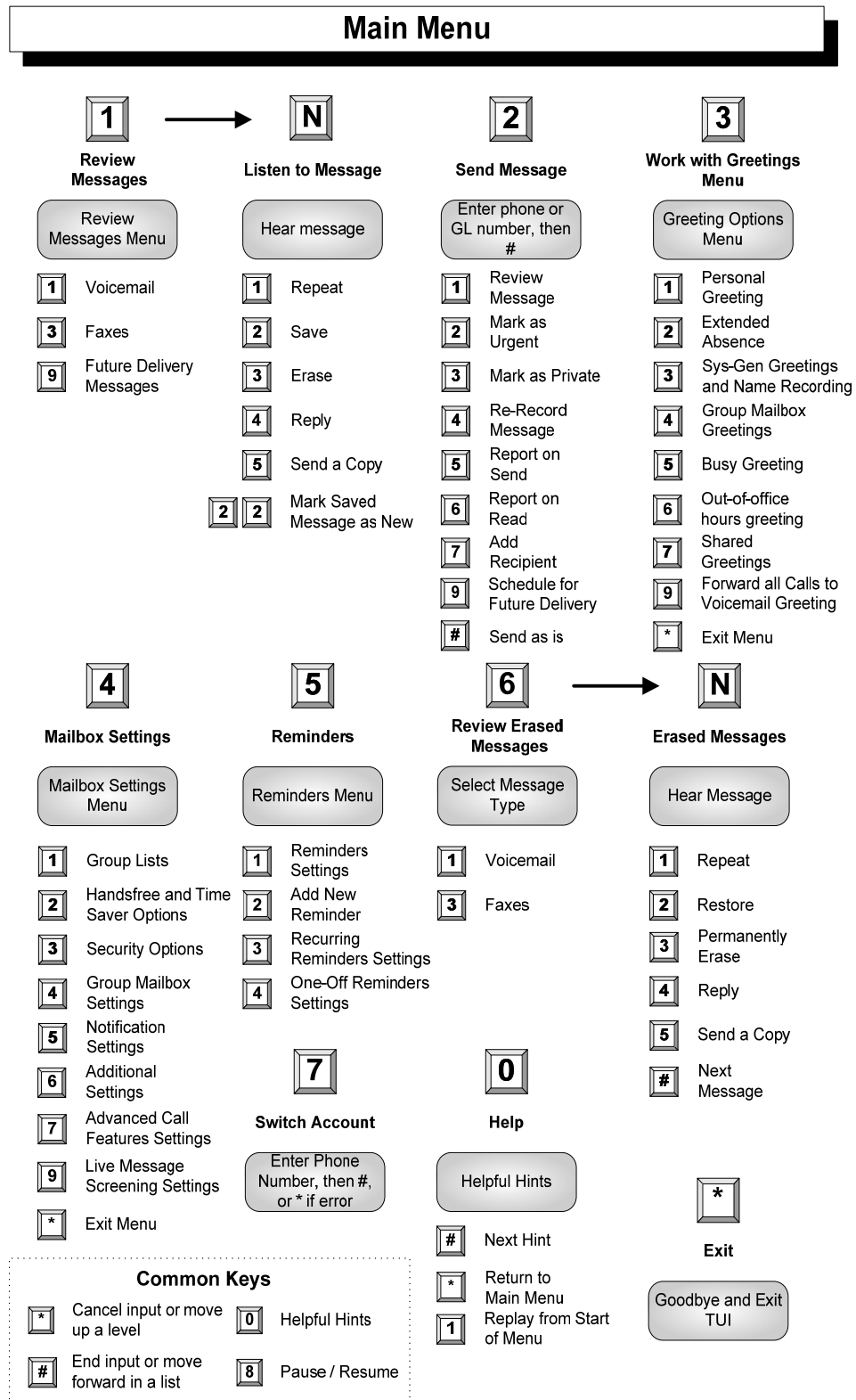
Figure 1: Main Menu
